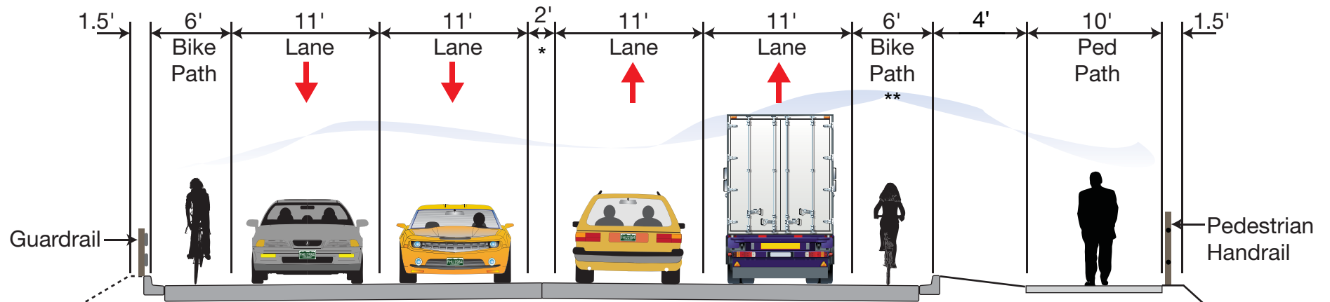
I-70G Typical Section Looking North
